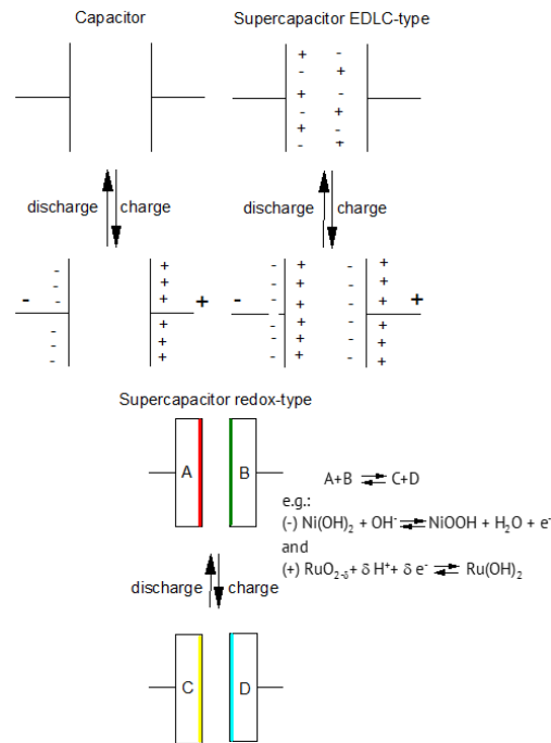
Figure 3. Charge distribution during operation in a conventional capacitor and in EDLC and redox-supercapacitors.
