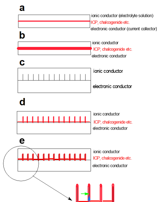
Figure 7. Sketches of electrode architectures.
