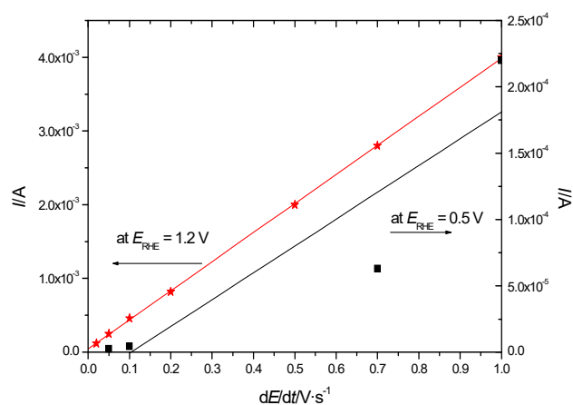
Figure 5. Current response vs. scan rate of a polycrystalline platinum electrode in contact with an aqueous electrolyte solution of 0.05 M \text{H}_2\text{SO}_4 , at different electrode potentials.
